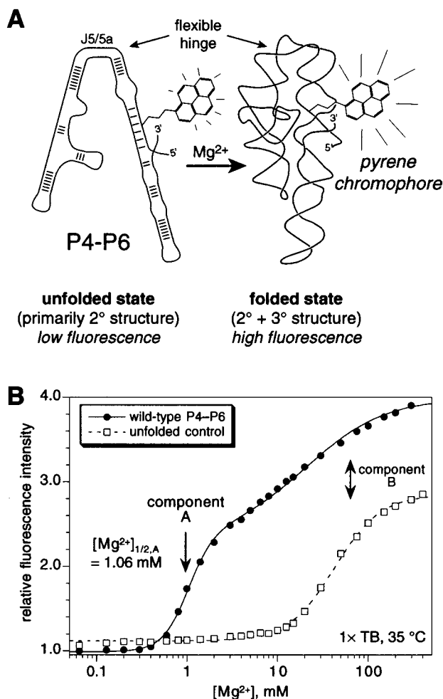
FIGURE 1: \text{Mg}^{2+} -dependent tertiary folding and equilibrium fluorescence titrations of pyrene-labeled P4–P6 RNA. (A) Schematic diagram of the tertiary folding of pyrene-labeled P4–P6. In the absence of \text{Mg}^{2+} , P4–P6 has secondary structure but little if any tertiary structure, and the fluorescence emission intensity of the covalently attached pyrene is low. Addition of \text{Mg}^{2+} induces tertiary folding, and the pyrene fluorescence emission intensity increases (36). (B) Equilibrium fluorescence titrations with \text{Mg}^{2+} of wild-type P4–P6 [P4–P6-wt-U107(pyr3)] and the unfolded control molecule P4–P6-bp [P4–P6-bp-U107(pyr3)], which is P4–P6 with several base substitutions in the J5/5a “hinge” region that establish Watson–Crick base pairing and thus lock the molecule into an unfolded conformation (34). The buffer was the standard Tris–borate buffer 1 \times TB (89 mM each Tris and boric acid, pH 8.3). Titrations were performed at 35 ^{\circ}\text{C} essentially as described (36) (see Materials and Methods). All data were fit as described (36). For wild-type pyrene-labeled P4–P6, the value of [\text{Mg}^{2+}]_{1/2,A} for component A was 1.06 \pm 0.02 mM ( n = 3 determinations; error = SEM), and the \text{Mg}^{2+} Hill coefficient n was 3.0 \pm 0.3 .
