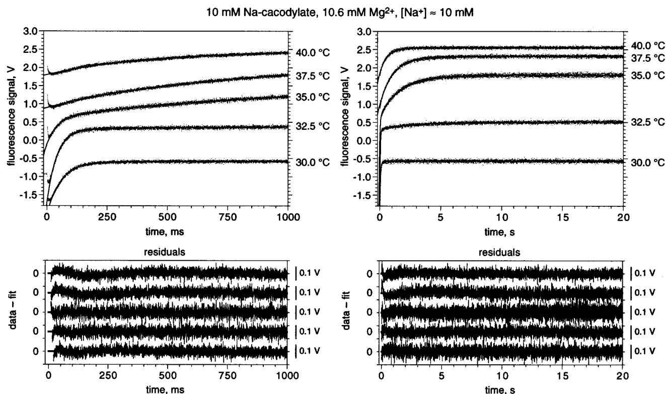
FIGURE 7: Strongly temperature-dependent switch between “fast” and “slow” kinetic phases for Mg 2+ -induced tertiary folding of P4–P6. Data were obtained between 30.0 and 40.0 °C in 10 mM sodium cacodylate, pH 7.5. The voltage origin for each trace is arbitrary; the traces are vertically offset for clarity. Note that the amplitude of voltage change for each trace is quantitatively similar. The data at 30.0, 37.5, and 40.0 °C were fit with single exponentials, while the data at 32.5 and 35.0 °C were fit with double exponentials. The only (fast) component at 30.0 °C was fit with k_{\text{obs}} = 17.0 \pm 0.1 \text{ s}^{-1} ( t_{1/2} = 40.8 \pm 0.2 \text{ ms} ). The kinetic values at 32.5 °C were fast component (92% of fluorescence change) k_{\text{obs}} = 24.2 \pm 0.1 \text{ s}^{-1} ( t_{1/2} = 28.6 \pm 0.2 \text{ ms} ) and slow component (8%) k_{\text{obs}} = 0.303 \pm 0.003 \text{ s}^{-1} ( t_{1/2} = 2.29 \pm 0.02 \text{ s} ). The data at 35.0 °C are the same as those shown in Figure 4. The only (slow) component at 37.5 °C was fit with k_{\text{obs}} = 0.930 \pm 0.004 \text{ s}^{-1} ( t_{1/2} = 745 \pm 4 \text{ ms} ), and at 40.0 °C with k_{\text{obs}} = 1.71 \pm 0.02 \text{ s}^{-1} ( t_{1/2} = 405 \pm 5 \text{ ms} ). Double-exponential fits to the 37.5 °C and 40.0 °C data did not improve the residuals (data not shown).
