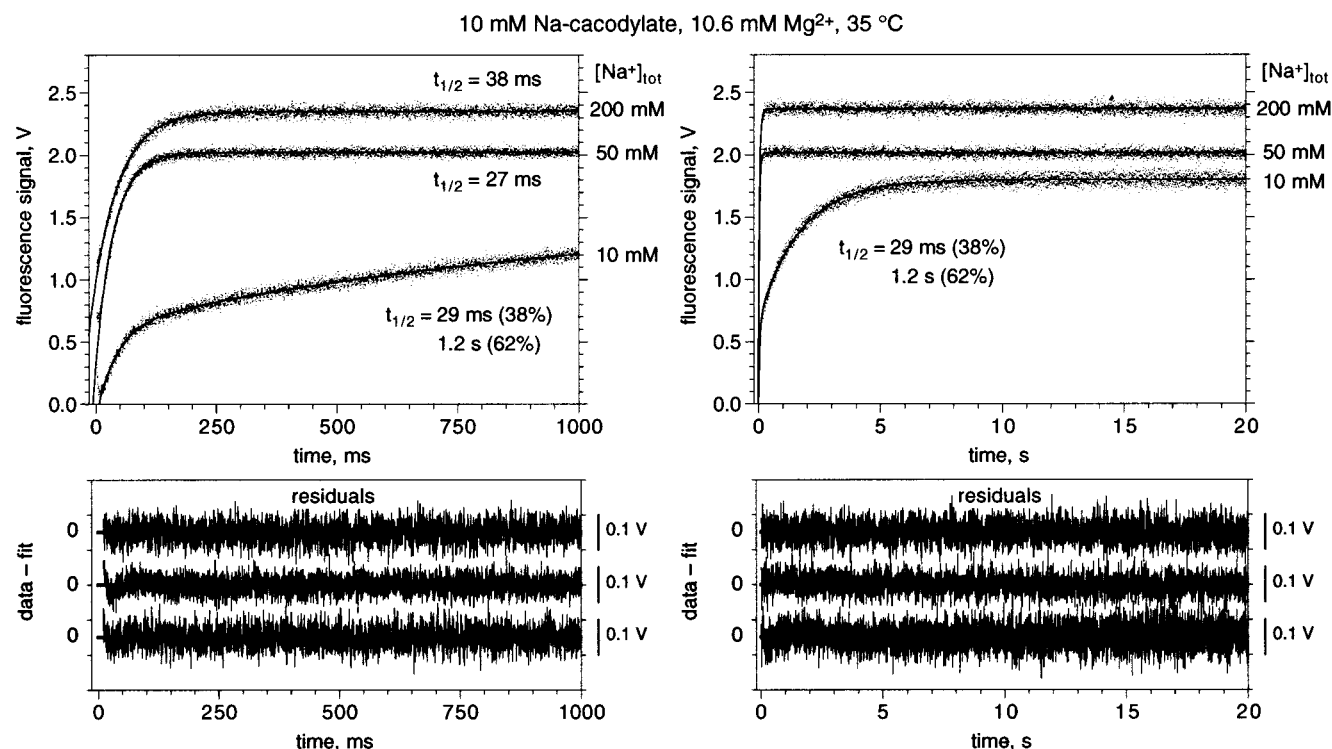
FIGURE 4: \text{Mg}^{2+} -induced folding of pyrene-labeled P4–P6 in sodium cacodylate buffer with varying [\text{Na}^+] . Data were collected as described in the Figure 2 caption. Three experiments are shown, in 10 mM sodium cacodylate buffer supplemented with NaCl to total [\text{Na}^+] of 10, 50, or 200 mM (i.e., 10 mM sodium cacodylate + 0, 40, or 190 mM NaCl). For each buffer, the left panel shows a kinetic trace obtained from 0 to 1000 ms after mixing, and the right panel shows data obtained from 0 to 20 s for the same sample. The voltage origin for each trace is arbitrary; the traces are vertically offset for clarity. Data at the lowest [\text{Na}^+] were fit with a double exponential with fast component (38% of fluorescence change) k_{\text{obs}} = 24.0 \pm 0.2 \text{ s}^{-1} ( t_{1/2} = 28.9 \pm 0.2 \text{ ms} ) [taken from left-panel data, 10–1000 ms] and slow component (62% of fluorescence change) k_{\text{obs}} = 0.585 \pm 0.004 \text{ s}^{-1} ( t_{1/2} = 1.18 \pm 0.01 \text{ s} ) [taken from right-panel data, 10 ms–20 s]. The ratio of components was 62% slow/38% fast for the illustrated data, but this varied somewhat depending on annealing conditions (38% slow for an unannealed sample) and on sample history (74% slow for a sample tested after processing through the stopped-flow experiment 18 times as described under Materials and Methods). In all such cases, however, the k_{\text{obs}} values were unchanged. Data at higher [\text{Na}^+] were fit with single exponentials.
